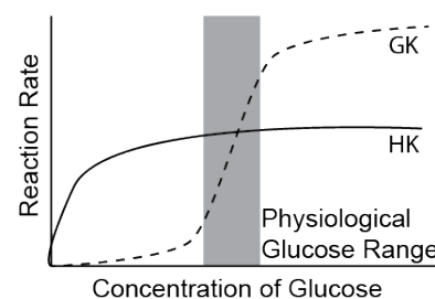
Figure 23: Schematic of the kinetics of glucokinase (GK) and hexokinase (HK). Note the differences in K_m , V_{max} and co-operativity between these enzymes.
